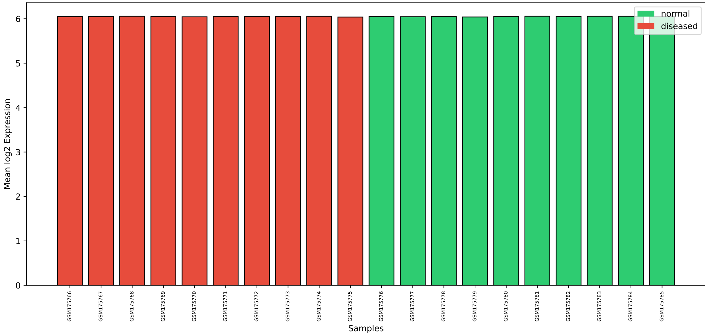
GSE7305: Endometriosis Dataset - Mean Expression
